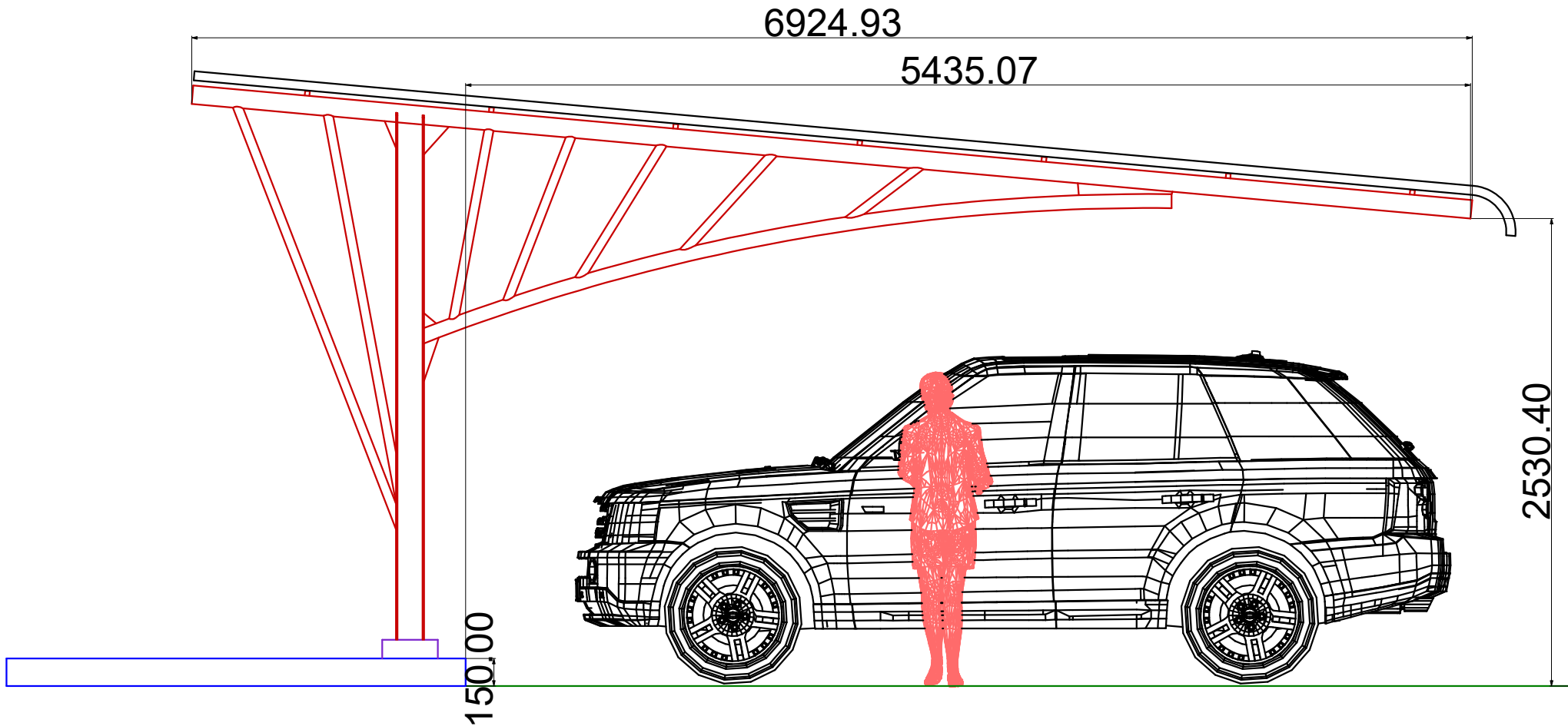
Proposed Parking Shade all dimensions in MM
